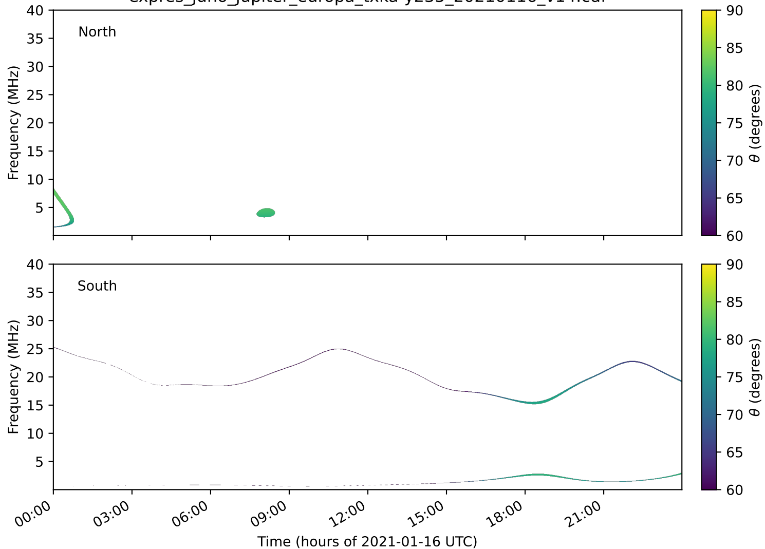
expres_juno_jupiter_europa_txka-y235_20210116_v14.cdf
