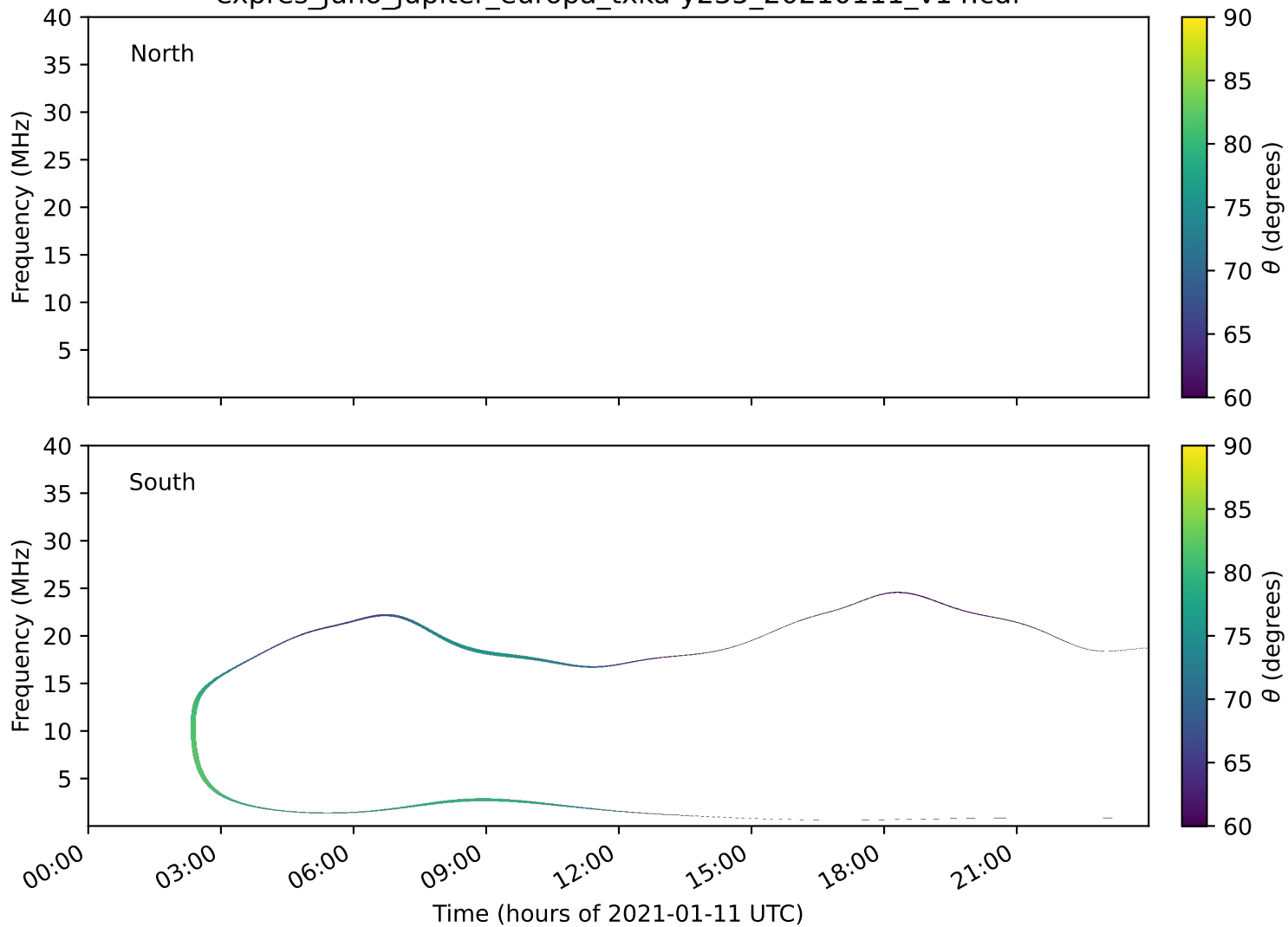
expres_juno_jupiter_europa_txka-y235_20210111_v14.cdf
