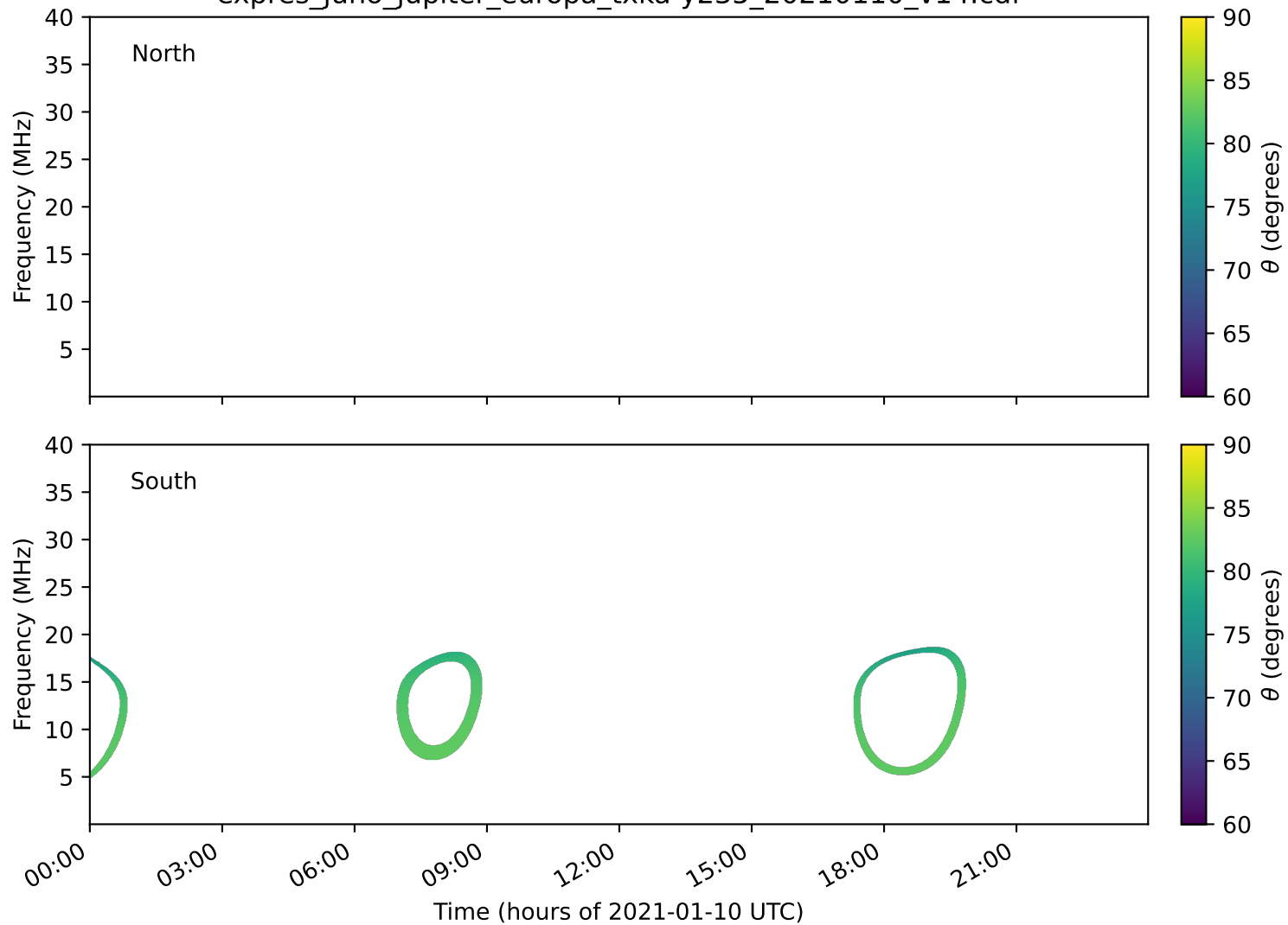
expres_juno_jupiter_europa_txka-y235_20210110_v14.cdf
