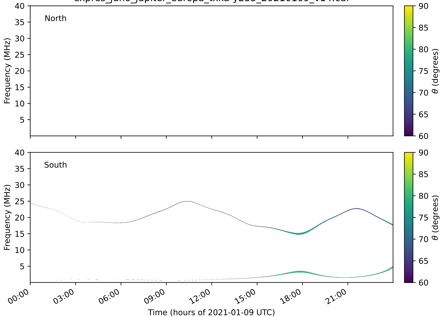
expres_juno_jupiter_europa_txka-y235_20210109_v14.cdf
