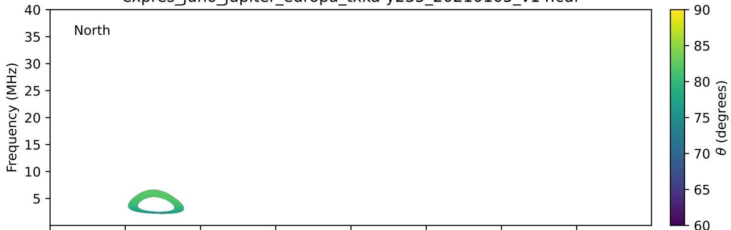
expres_juno_jupiter_europa_txka-y235_20210105_v14.cdf
