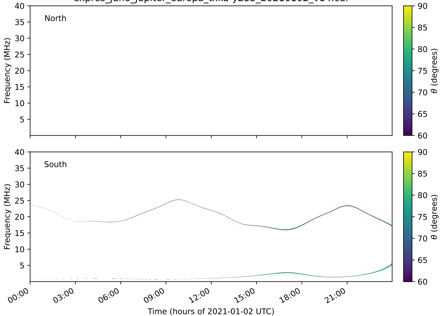
expres_juno_jupiter_europa_txka-y235_20210102_v14.cdf
