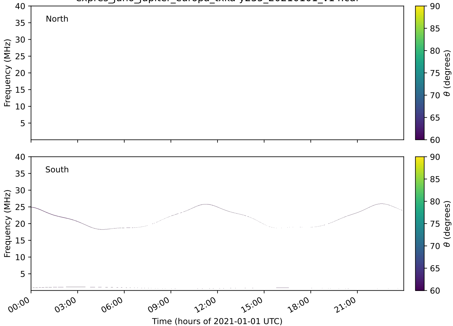
expres_juno_jupiter_europa_txka-y235_20210101_v14.cdf
