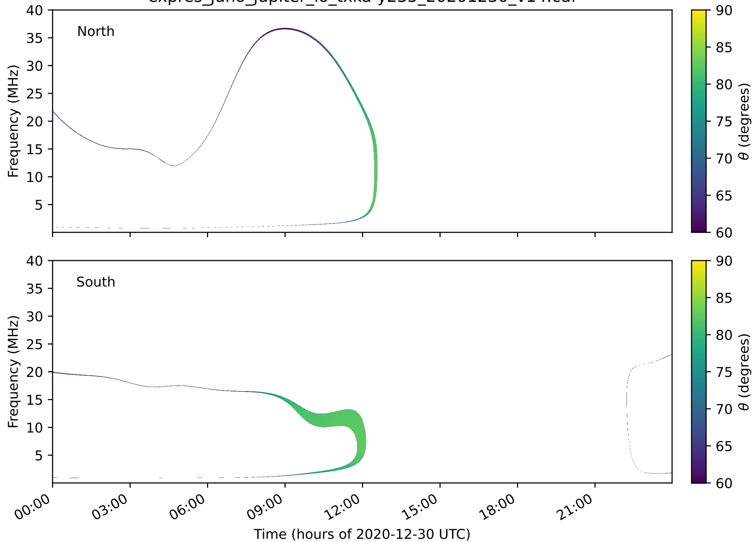
expres_juno_jupiter_io_txka-y235_20201230_v14.cdf
