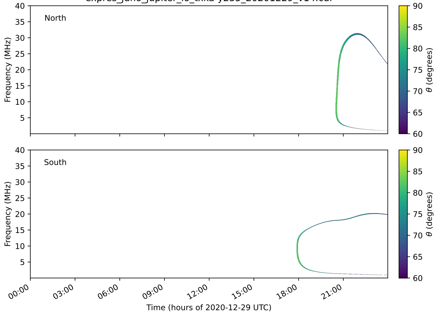
expres_juno_jupiter_io_txka-y235_20201229_v14.cdf
