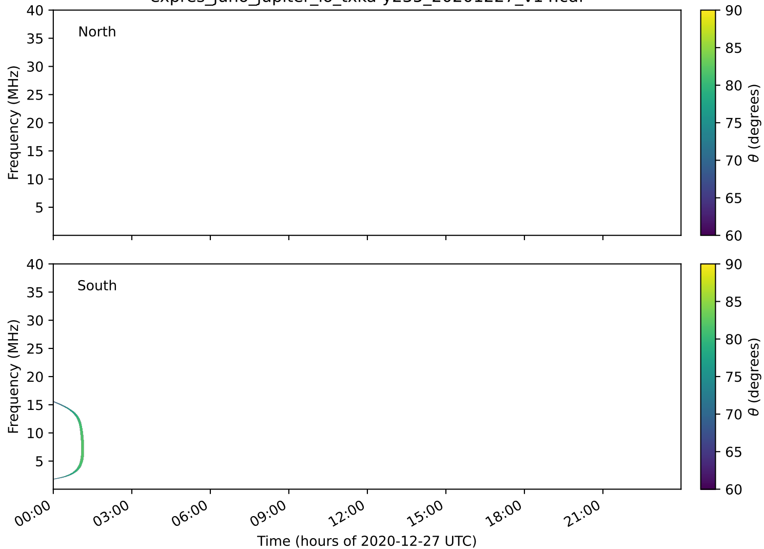
expres_juno_jupiter_io_txka-y235_20201227_v14.cdf
