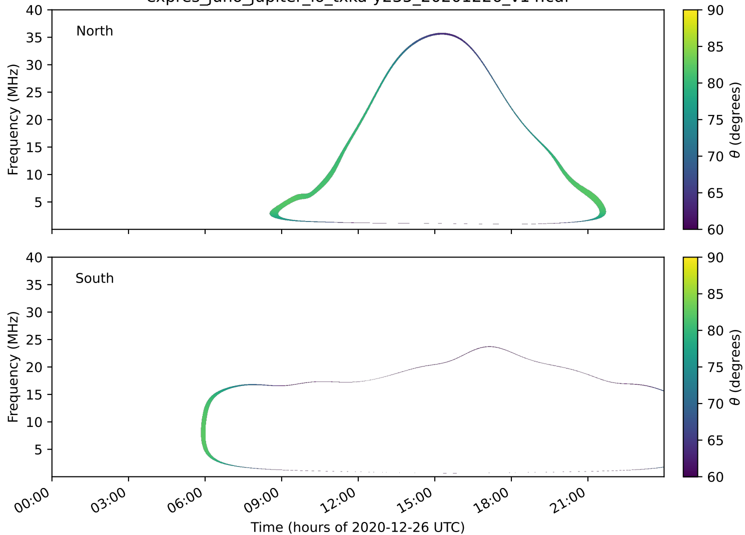
expres_juno_jupiter_io_txka-y235_20201226_v14.cdf
