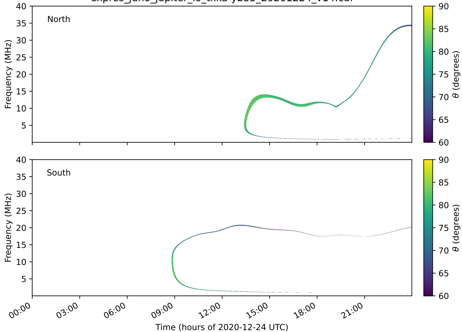
expres_juno_jupiter_io_txka-y235_20201224_v14.cdf
