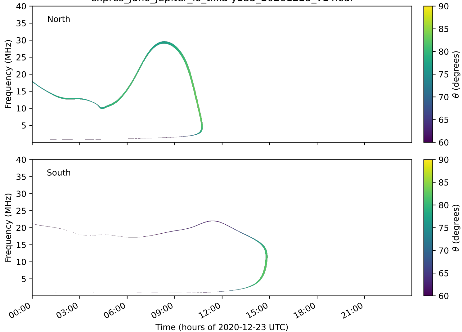
expres_juno_jupiter_io_txka-y235_20201223_v14.cdf
