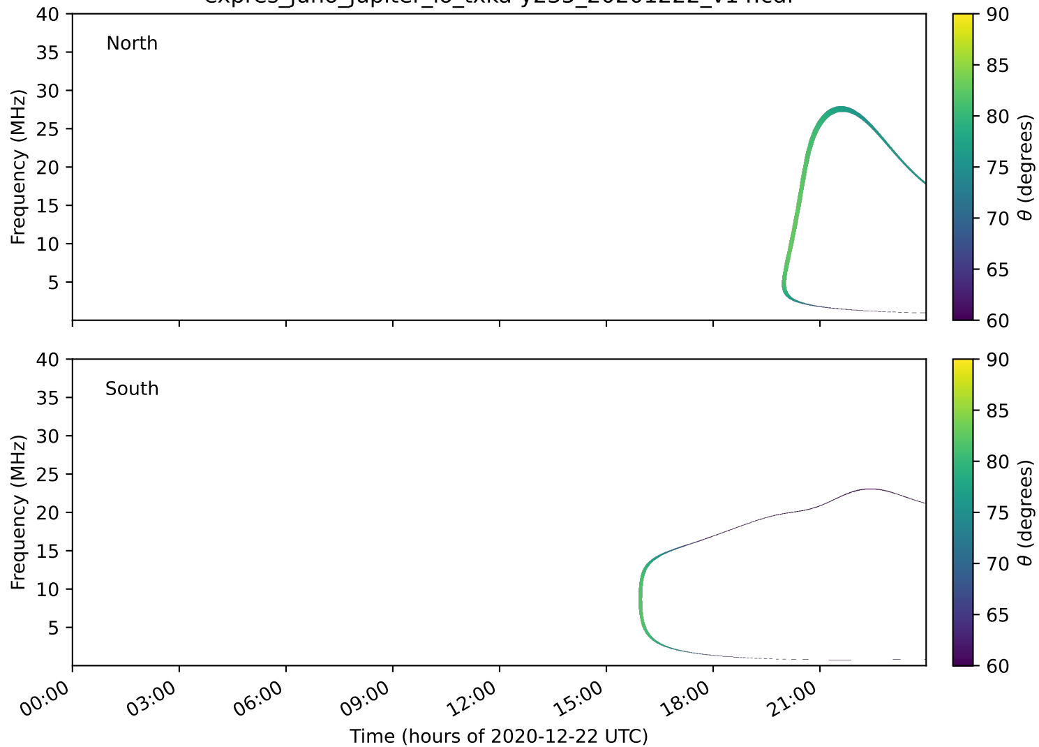
expres_juno_jupiter_io_txka-y235_20201222_v14.cdf
