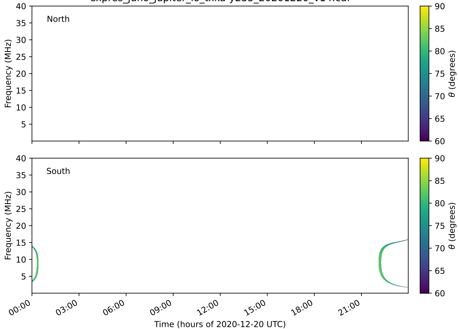
expres_juno_jupiter_io_txka-y235_20201220_v14.cdf
