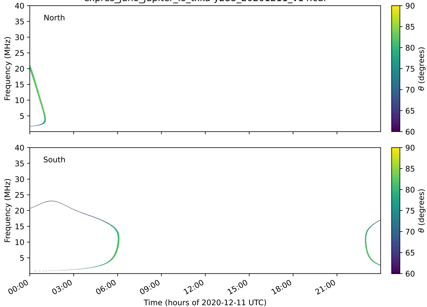
expres_juno_jupiter_io_txka-y235_20201211_v14.cdf
