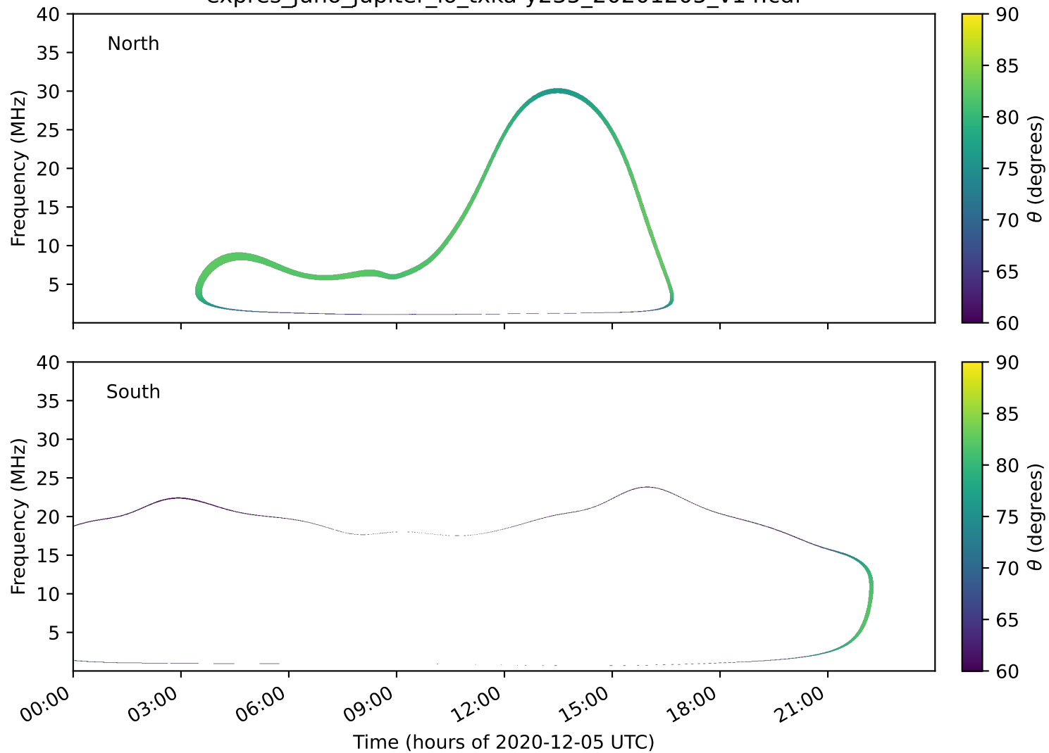
expres_juno_jupiter_io_txka-y235_20201205_v14.cdf
