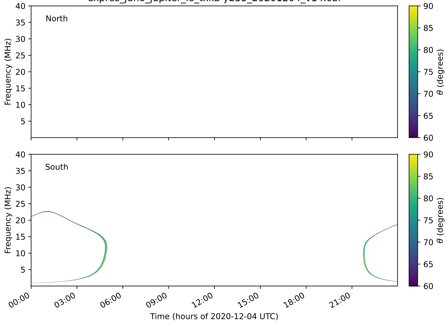
expres_juno_jupiter_io_txka-y235_20201204_v14.cdf
