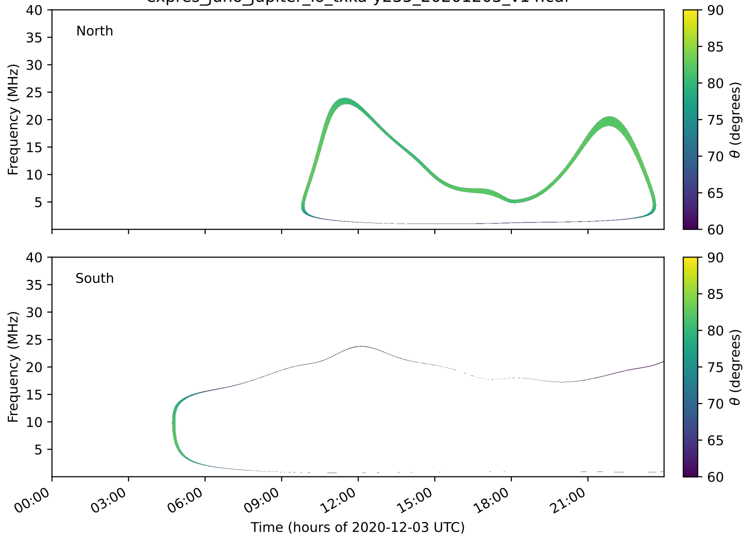
expres_juno_jupiter_io_txka-y235_20201203_v14.cdf
