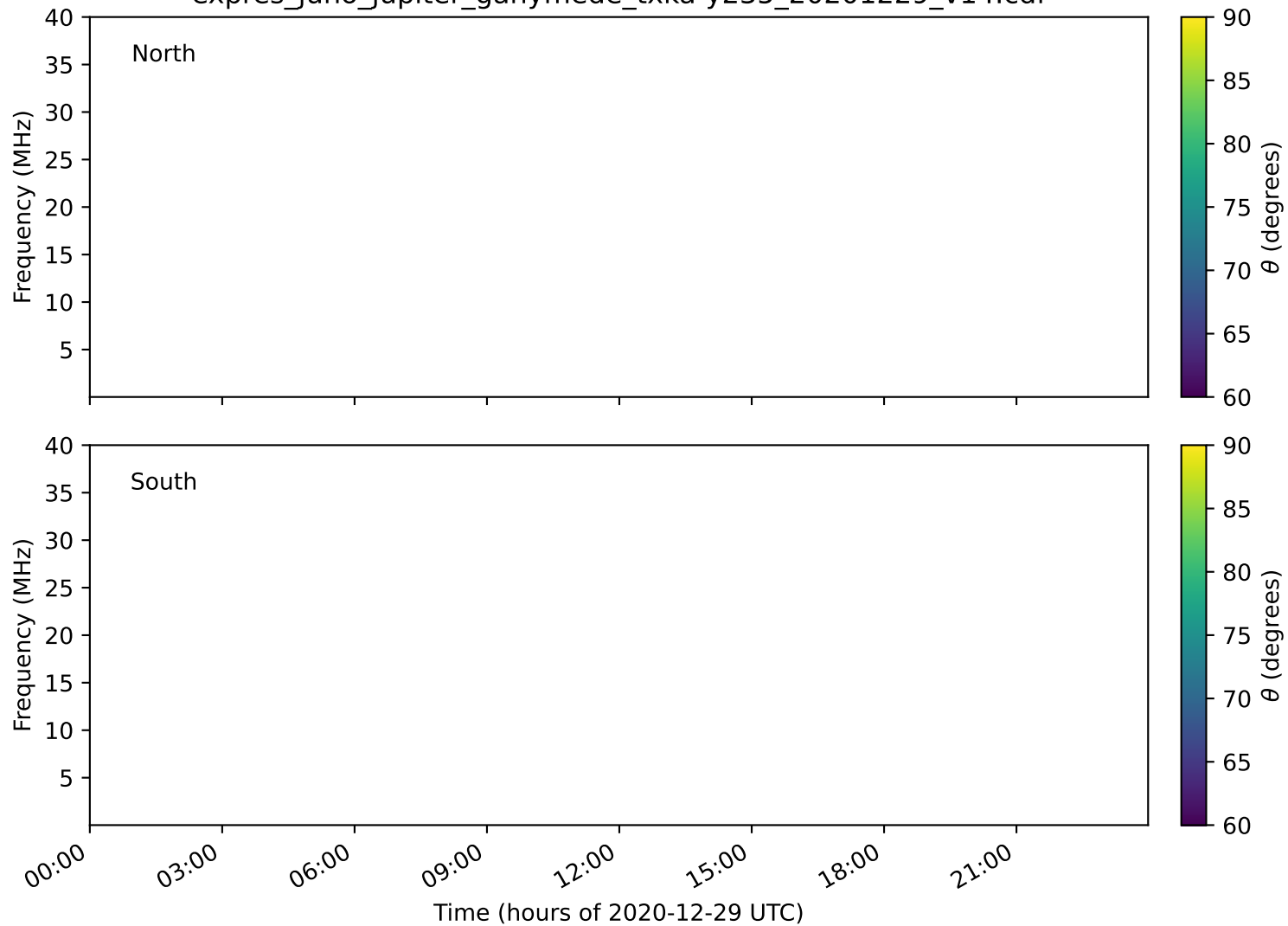
expres_juno_jupiter_ganymede_txka-y235_20201229_v14.cdf
