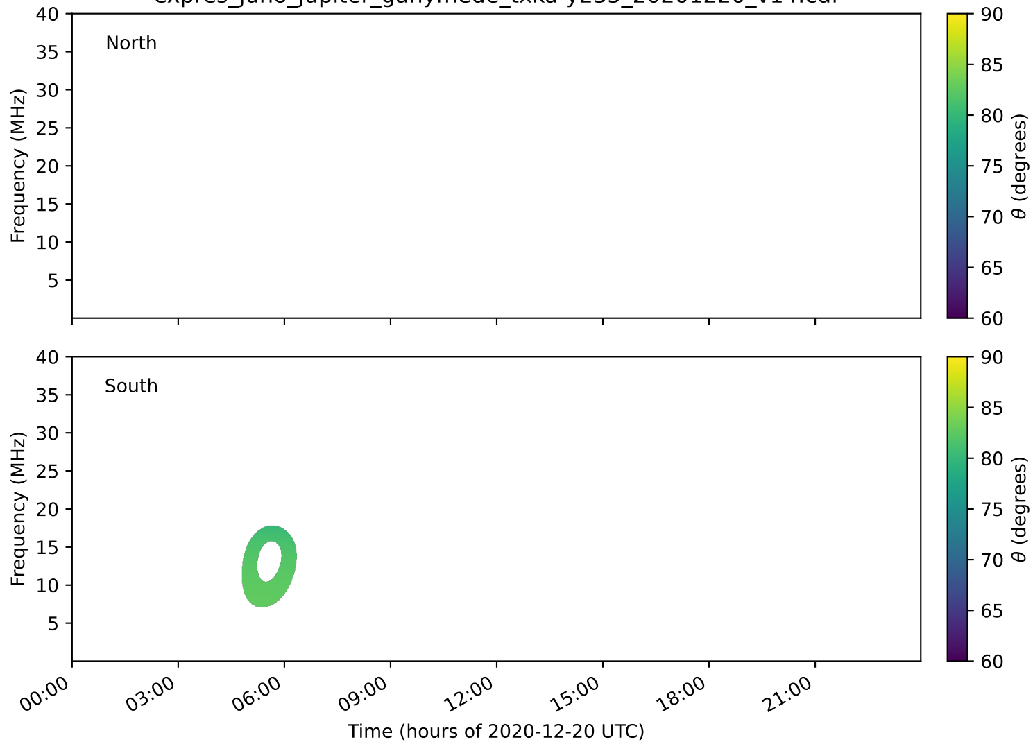
expres_juno_jupiter_ganymede_txka-y235_20201220_v14.cdf
