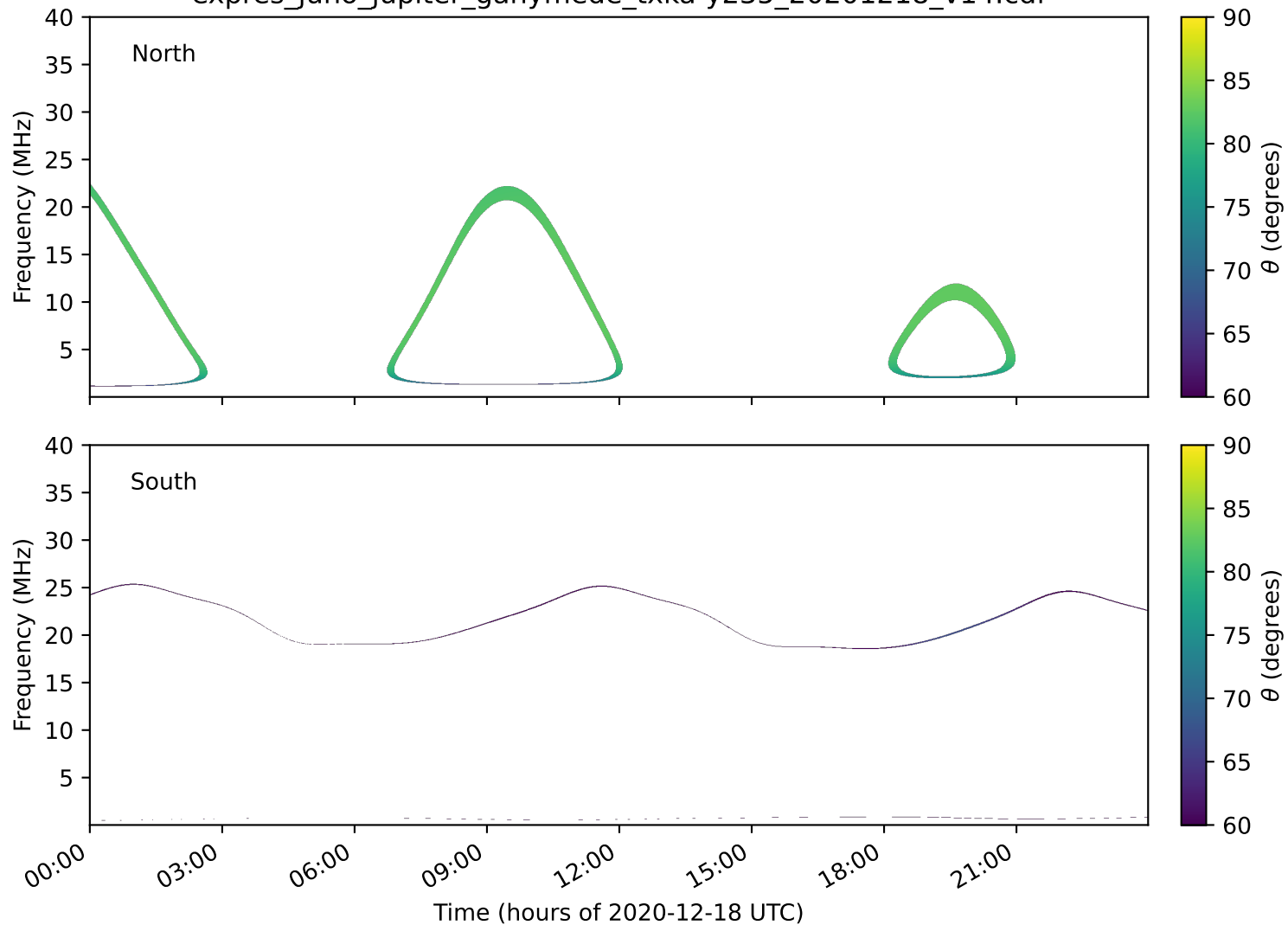
expres_juno_jupiter_ganymede_txka-y235_20201218_v14.cdf
