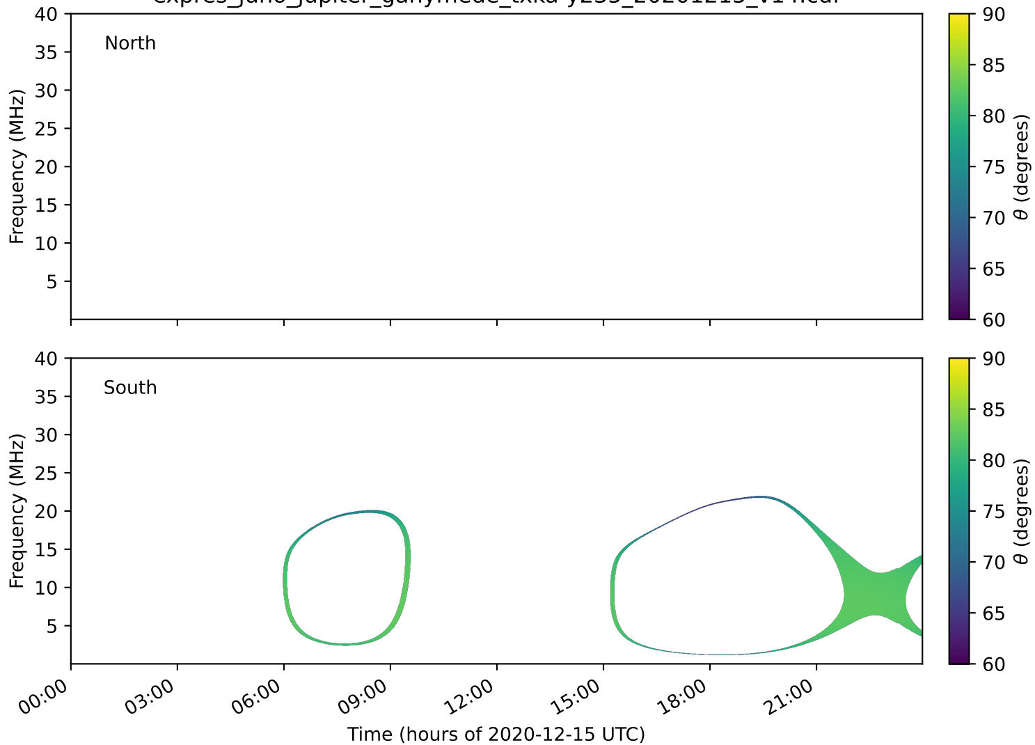
expres_juno_jupiter_ganymede_txka-y235_20201215_v14.cdf
