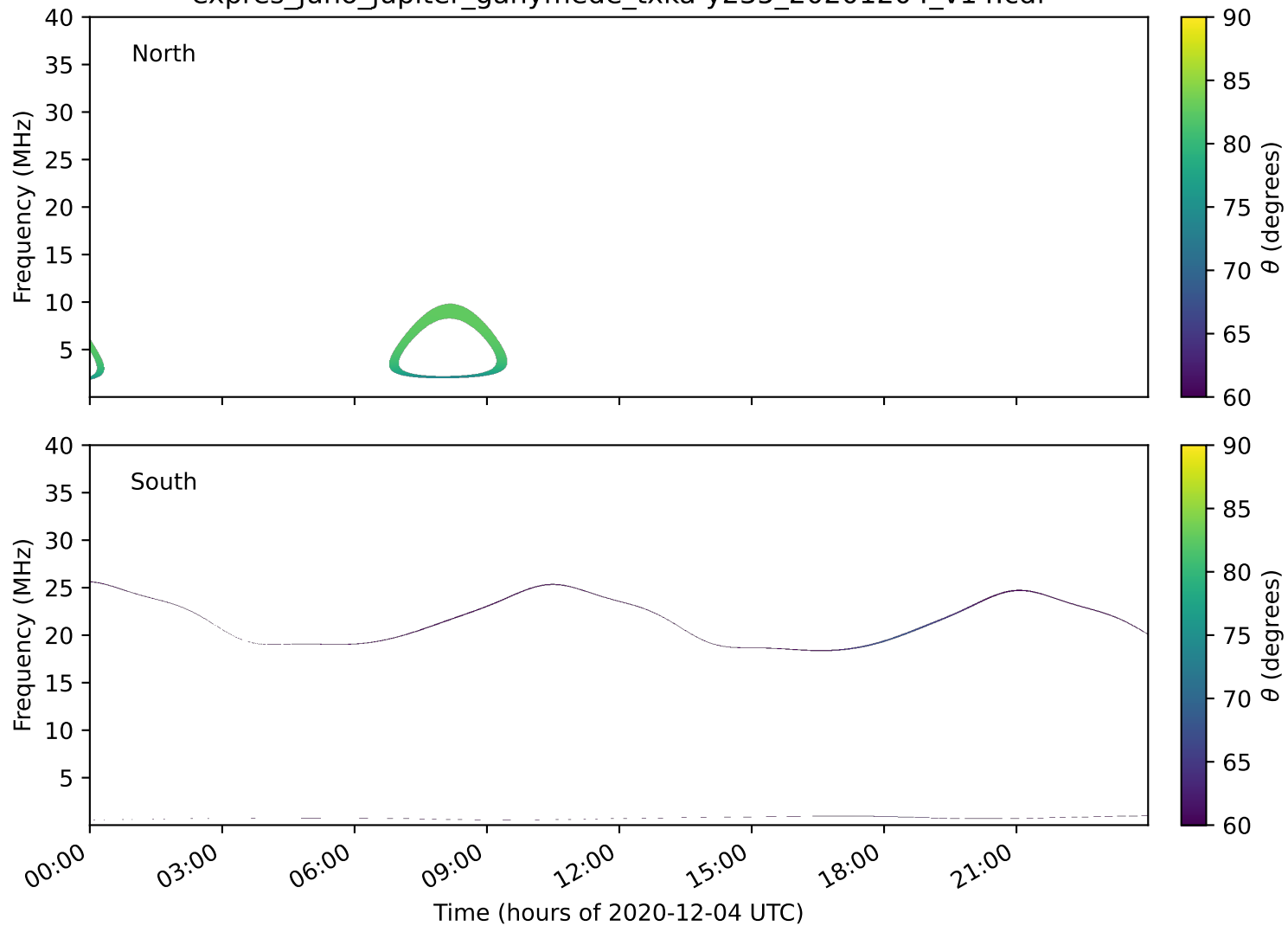
expres_juno_jupiter_ganymede_txka-y235_20201204_v14.cdf
