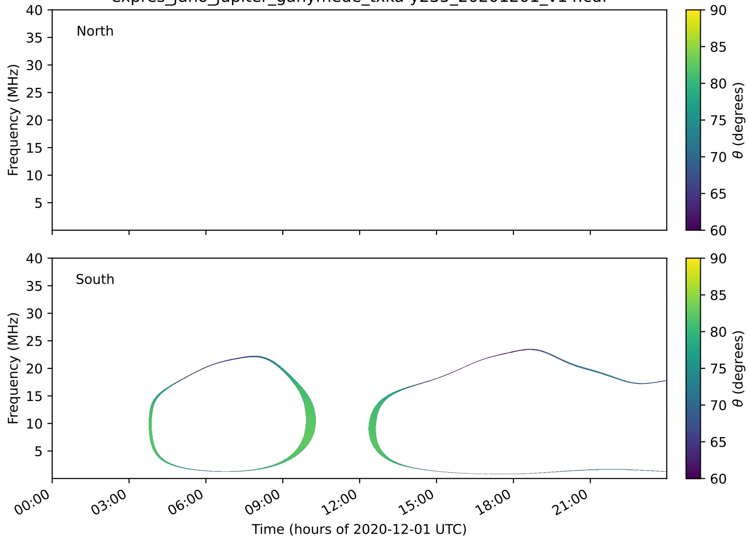
expres_juno_jupiter_ganymede_txka-y235_20201201_v14.cdf
