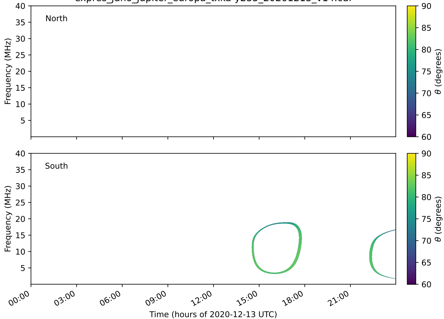
expres_juno_jupiter_europa_txka-y235_20201213_v14.cdf
