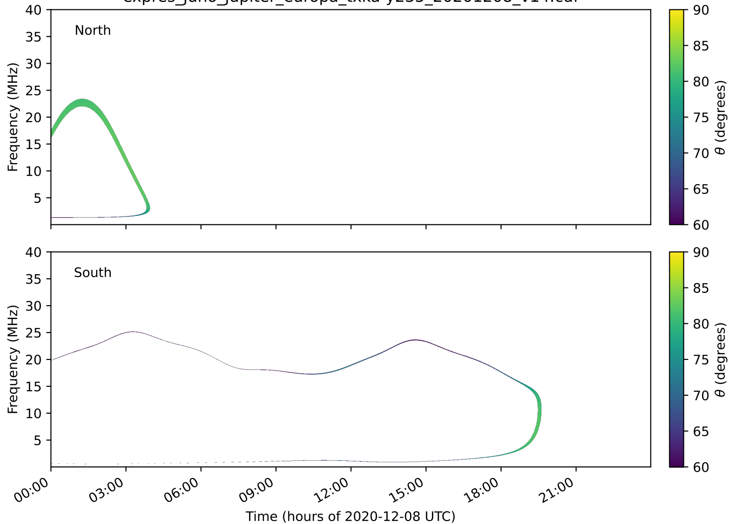
expres_juno_jupiter_europa_txka-y235_20201208_v14.cdf
