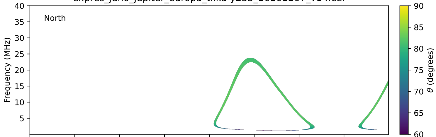
expres_juno_jupiter_europa_txka-y235_20201207_v14.cdf
