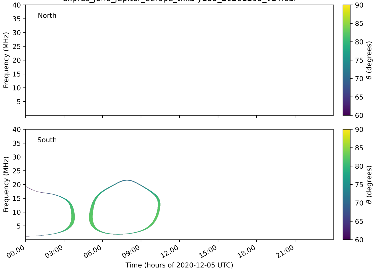
expres_juno_jupiter_europa_txka-y235_20201205_v14.cdf
