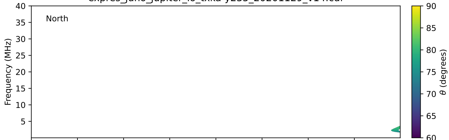
expres_juno_jupiter_io_txka-y235_20201129_v14.cdf
