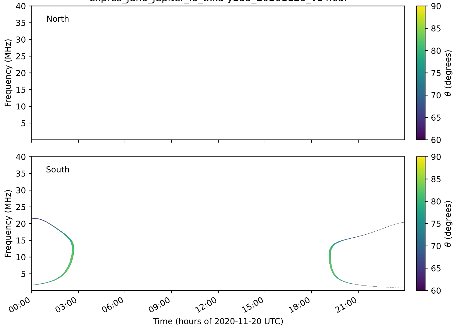
expres_juno_jupiter_io_txka-y235_20201120_v14.cdf
