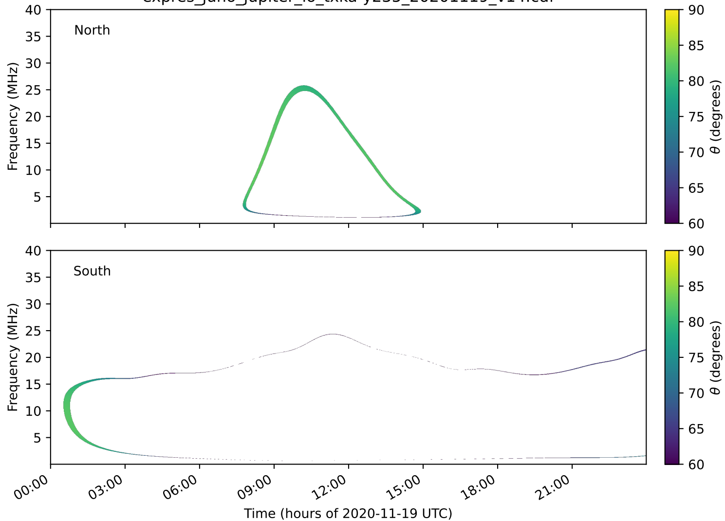
expres_juno_jupiter_io_txka-y235_20201119_v14.cdf
