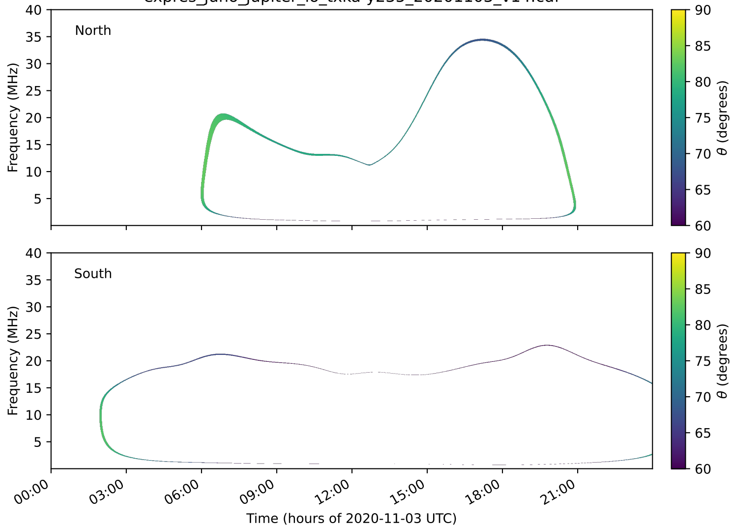
expres_juno_jupiter_io_txka-y235_20201103_v14.cdf
