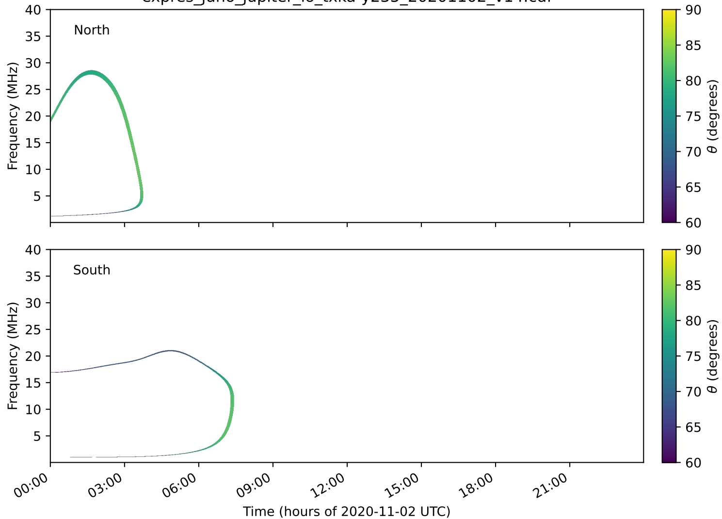
expres_juno_jupiter_io_txka-y235_20201102_v14.cdf
