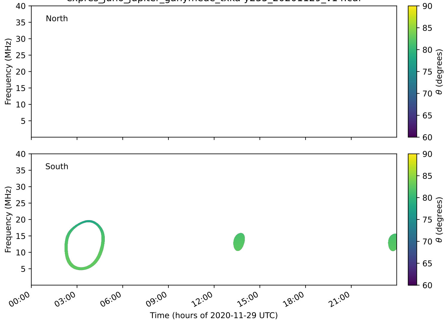
expres_juno_jupiter_ganymede_txka-y235_20201129_v14.cdf
