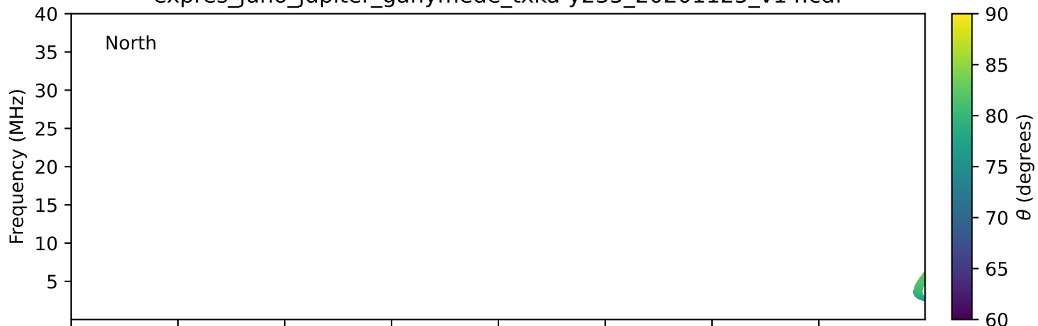
expres_juno_jupiter_ganymede_txka-y235_20201125_v14.cdf
