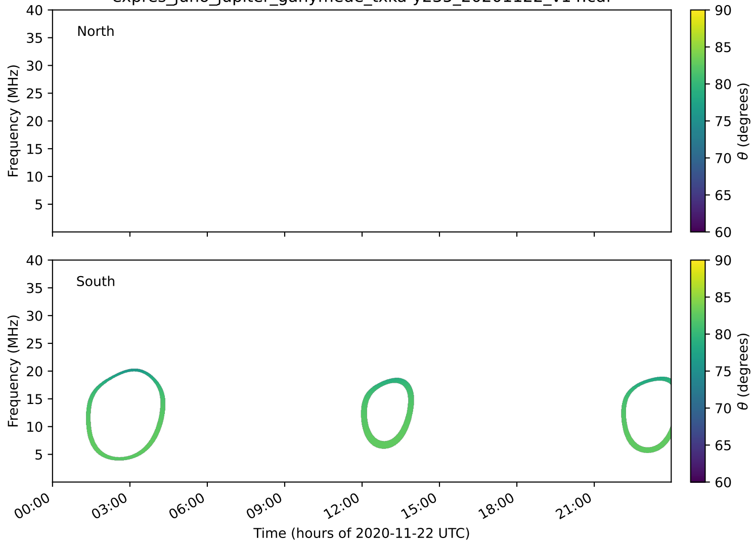
expres_juno_jupiter_ganymede_txka-y235_20201122_v14.cdf
