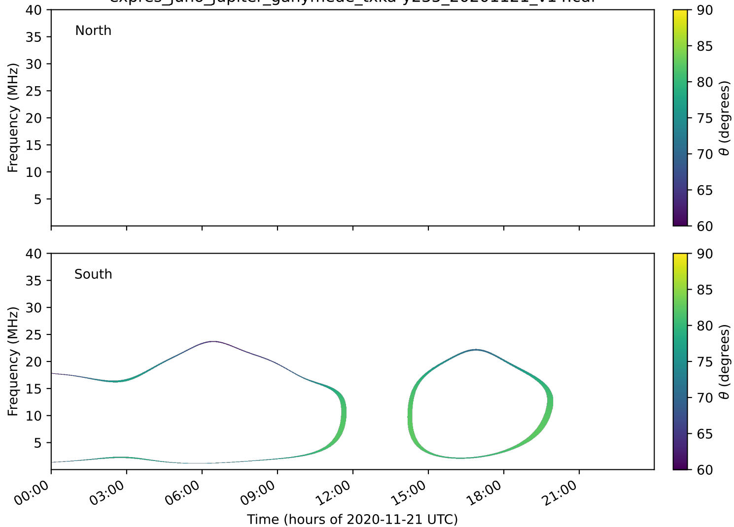
expres_juno_jupiter_ganymede_txka-y235_20201121_v14.cdf
