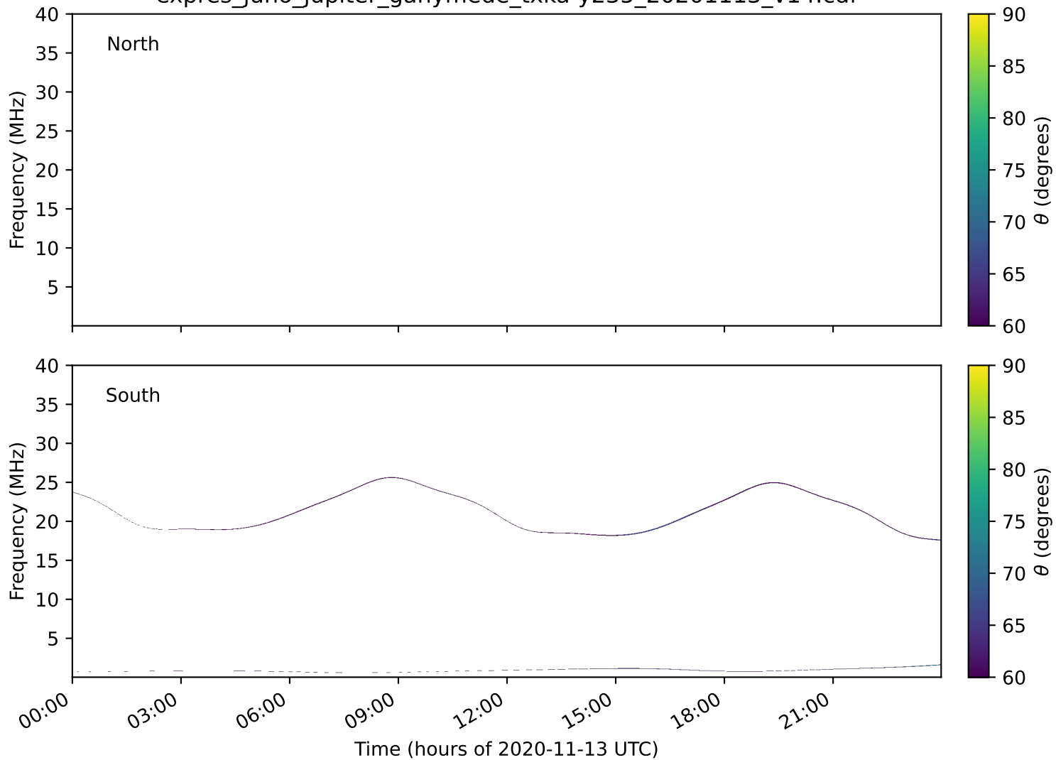
expres_juno_jupiter_ganymede_txka-y235_20201113_v14.cdf
