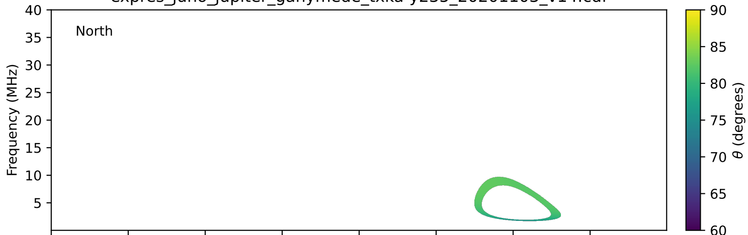
expres_juno_jupiter_ganymede_txka-y235_20201103_v14.cdf
