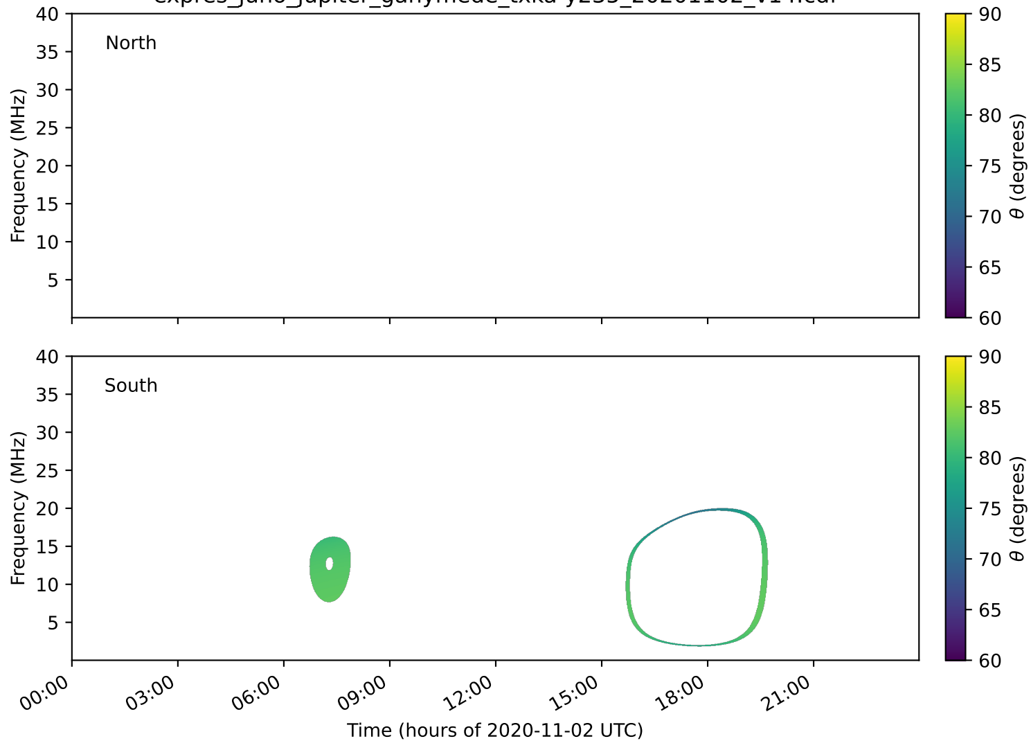
expres_juno_jupiter_ganymede_txka-y235_20201102_v14.cdf
