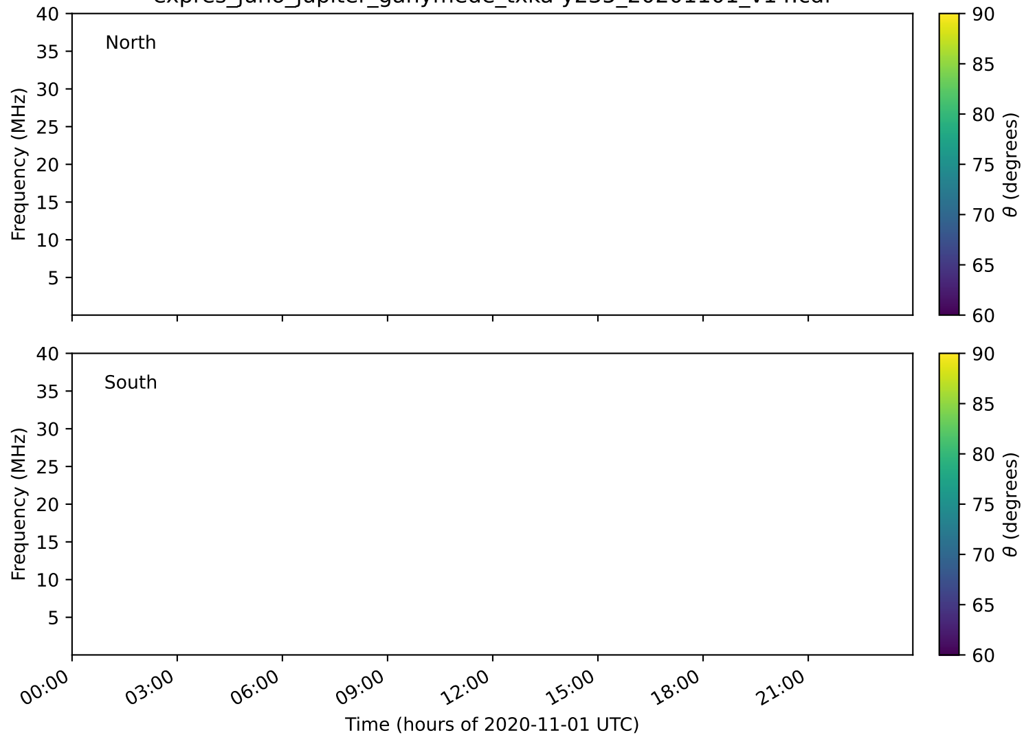
expres_juno_jupiter_ganymede_txka-y235_20201101_v14.cdf
