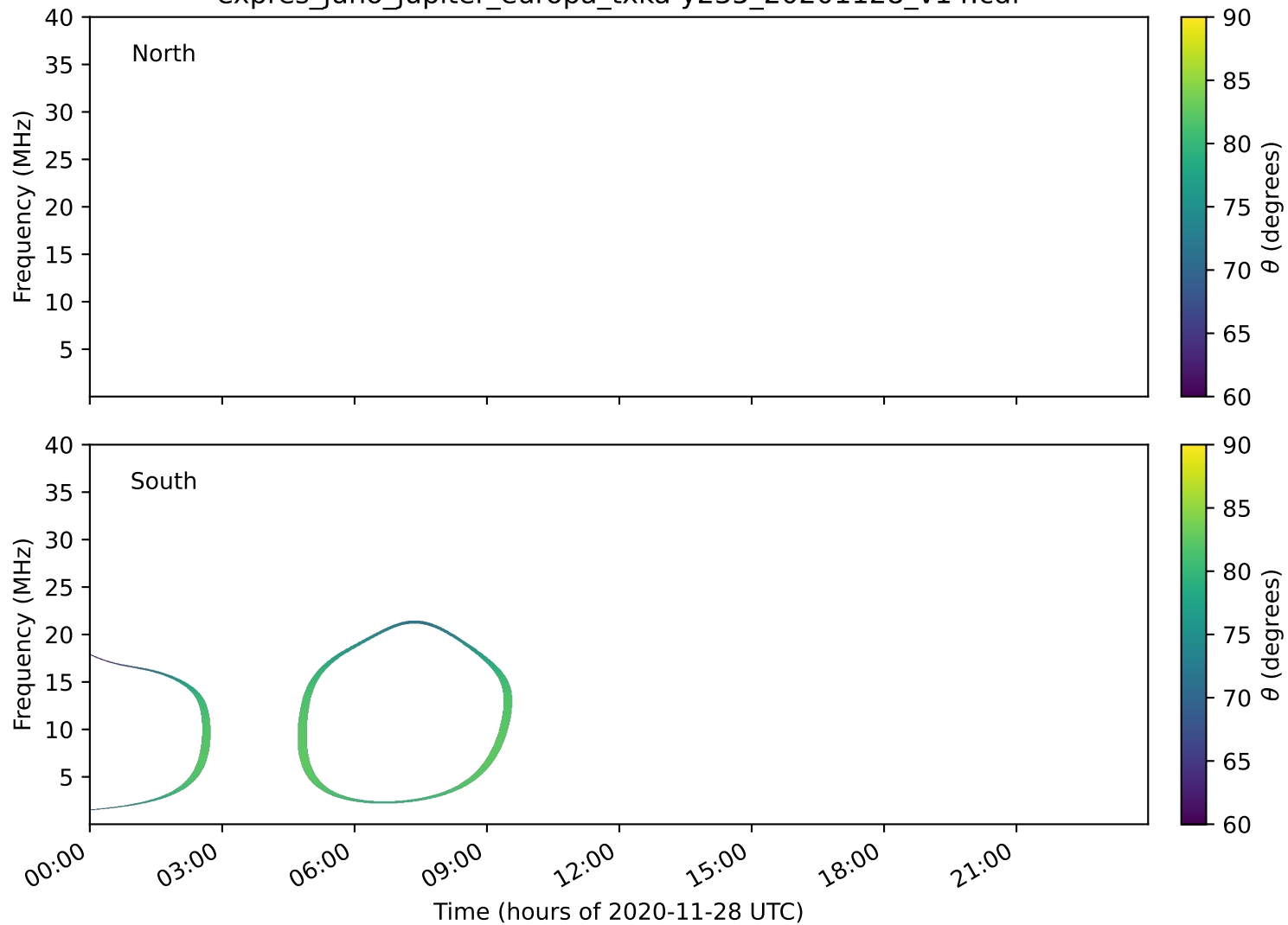
expres_juno_jupiter_europa_txka-y235_20201128_v14.cdf
