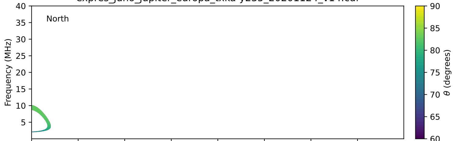
expres_juno_jupiter_europa_txka-y235_20201124_v14.cdf
