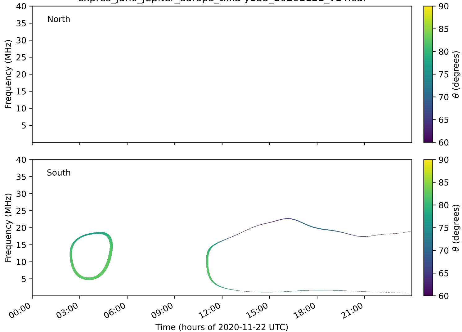
expres_juno_jupiter_europa_txka-y235_20201122_v14.cdf
