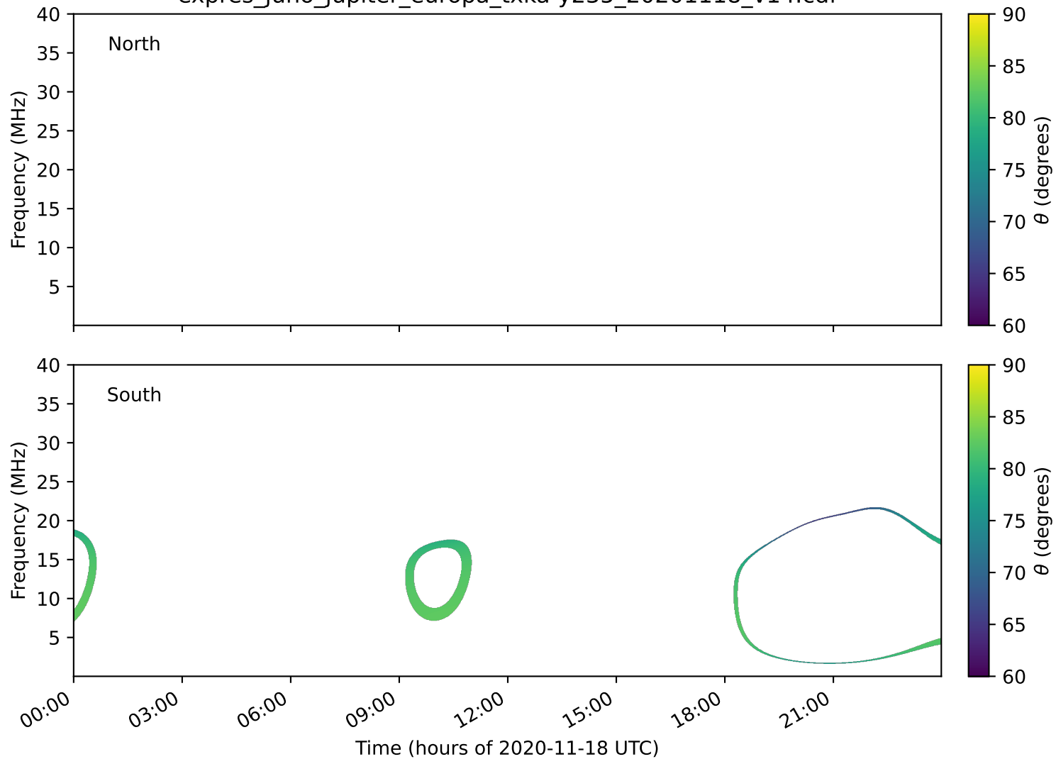
expres_juno_jupiter_europa_txka-y235_20201118_v14.cdf
