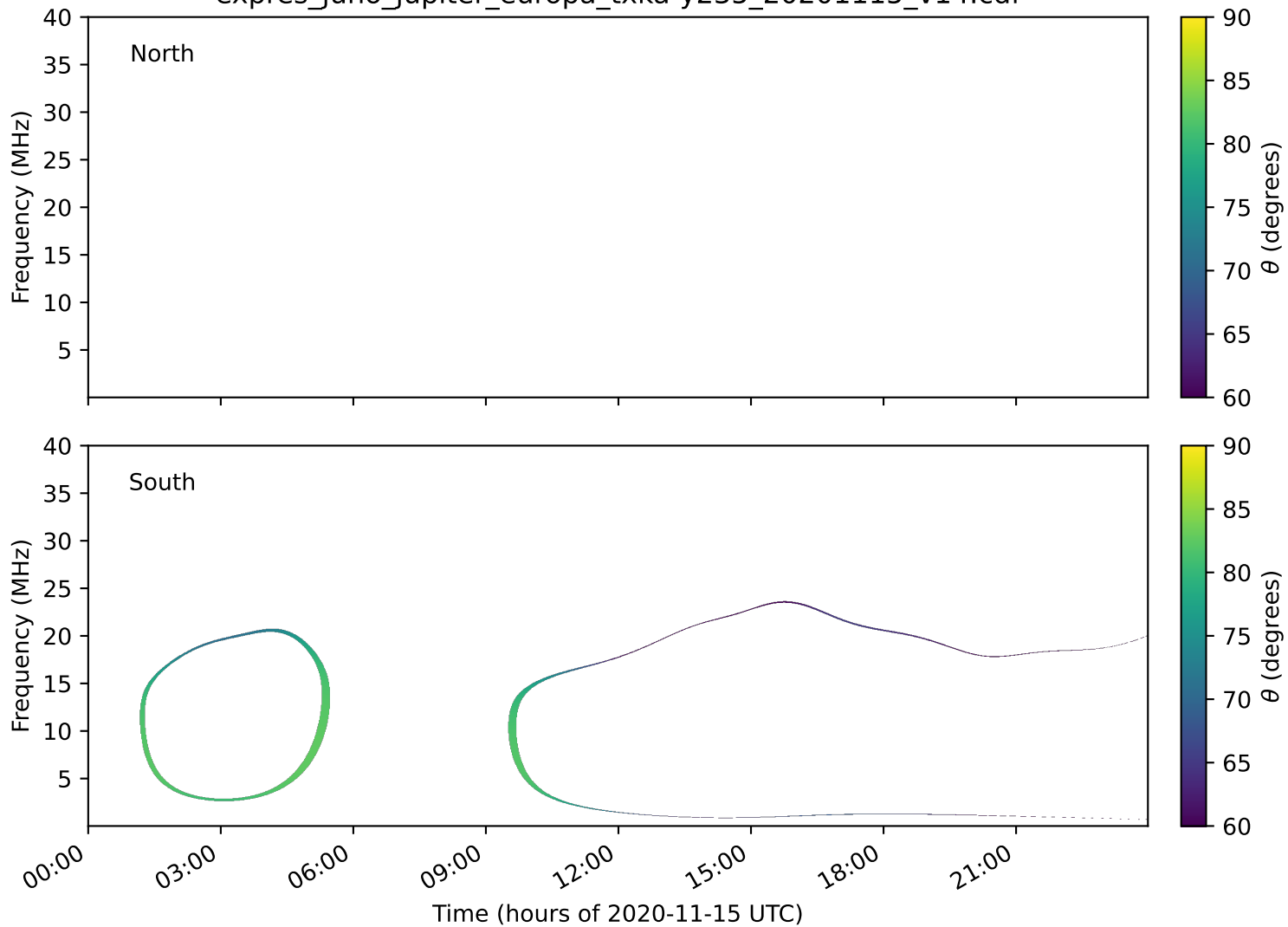
expres_juno_jupiter_europa_txka-y235_20201115_v14.cdf
