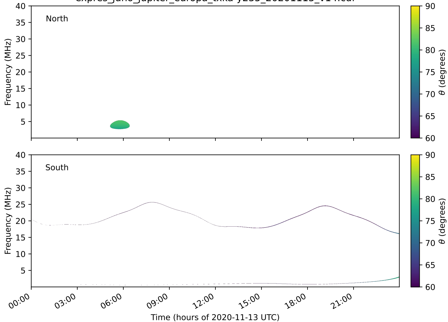
expres_juno_jupiter_europa_txka-y235_20201113_v14.cdf
