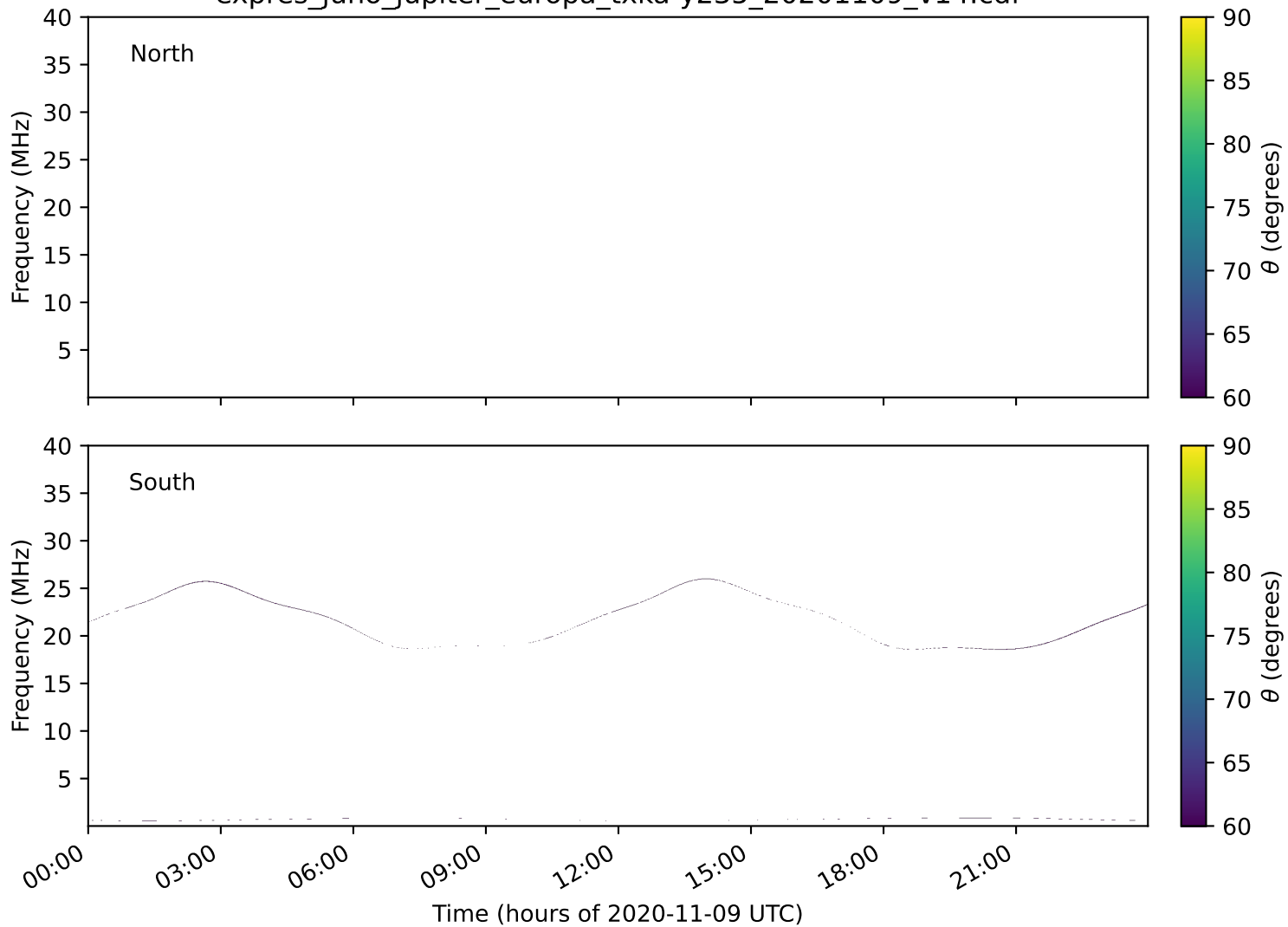
expres_juno_jupiter_europa_txka-y235_20201109_v14.cdf
