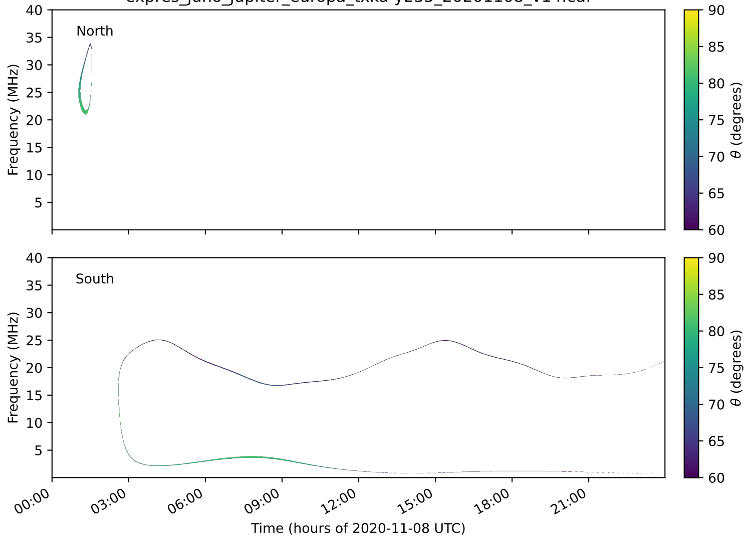
expres_juno_jupiter_europa_txka-y235_20201108_v14.cdf
